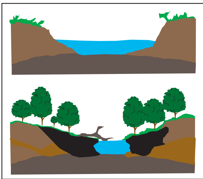
Figure 5. Comparison of stream banks with and without riparian vegetation (adapted from Pritchard 1998.)
