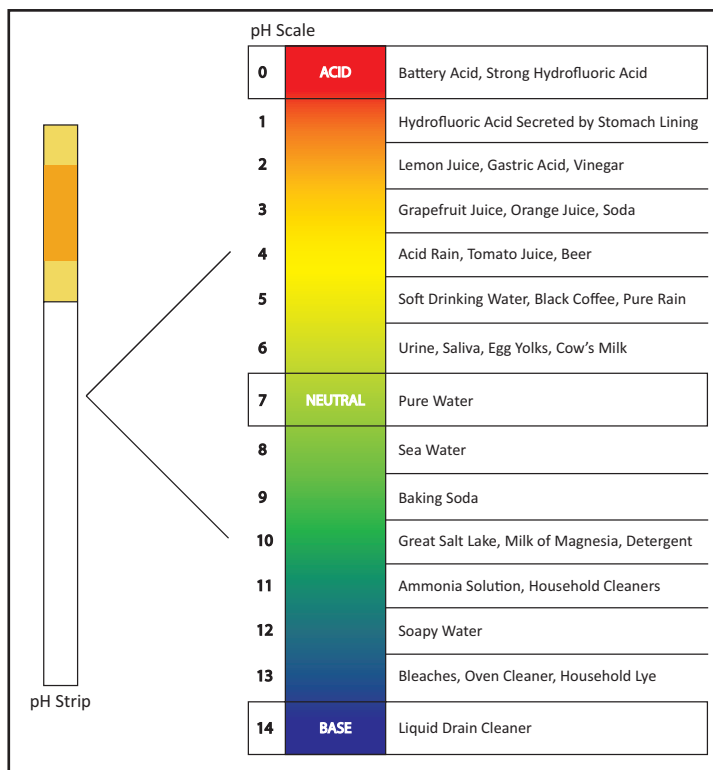
Figure 11. pH strip and pH scale.
