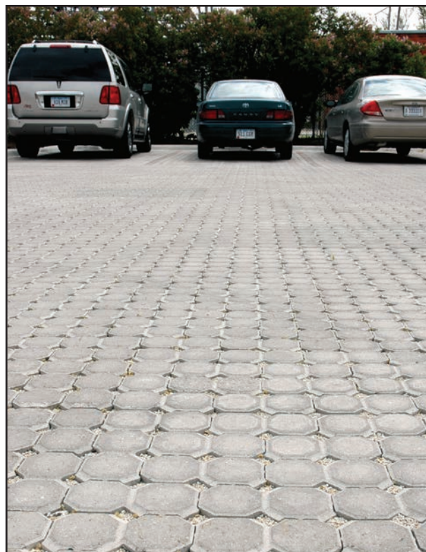
Figure 38. A porous pavement system in a shopping mall parking lot. (Photo courtesy of USDA Natural Resources Conservation Service.)
