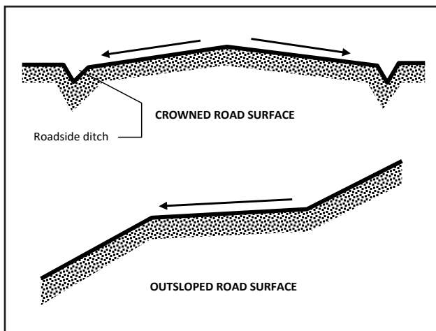
Figure 48. Cross sectional profiles of crowned and outsloped road surfaces for effective drainage. (Diagram courtesy of the Texas Forest Service.)
