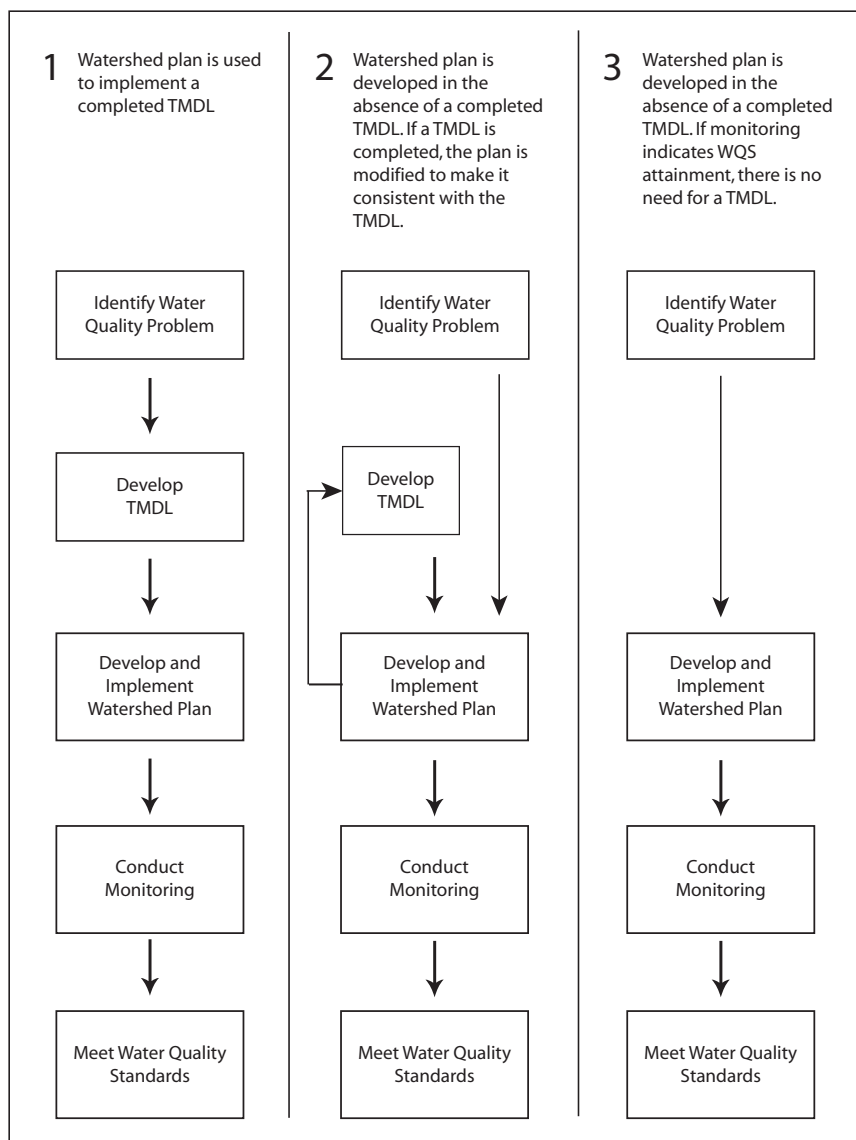
Figure 26. Potential relationships between TMDLs and watershed plans (WPPs). (Adapted from Figure 2-2 in Handbook for Developing Watershed Plans to Restore and Protect Our Waters, EPA, 2005.)
